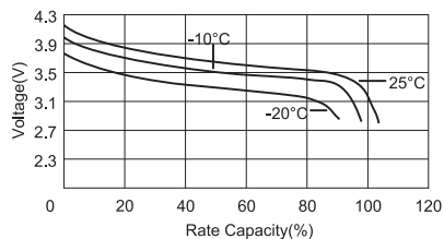
Temperature Characteristics
