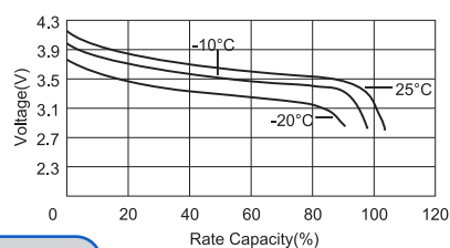
Temperature Characteristics
