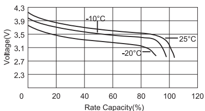
Temperature Characteristics
