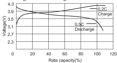
Charge and Discharge Characteristics
