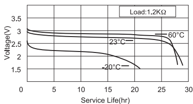
Temperature Characteristics
