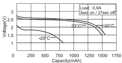
Pulse Discharge Characteristics
