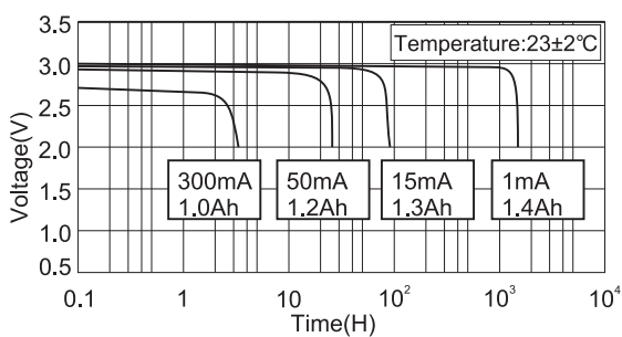
Discharge Characteristics
