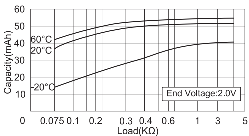
Load-capacity
