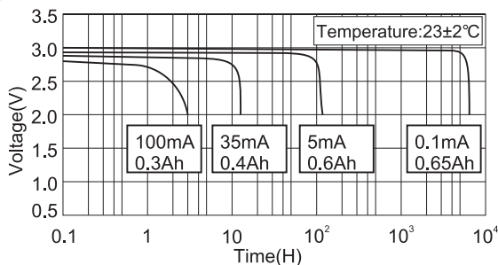
Discharge Characteristics
