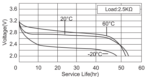
Temperature Characteristics
