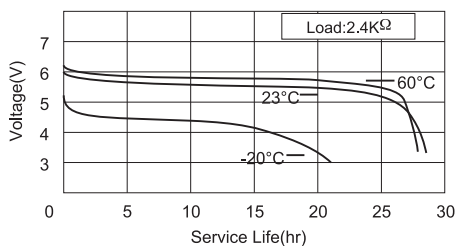
Temperature Characteristic
