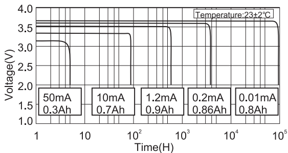
Discharge Characteristics
