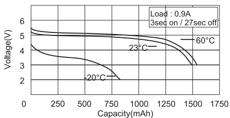
Pulse Discharge Characteristics
